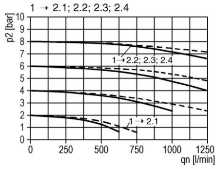
flow characteristic 2
